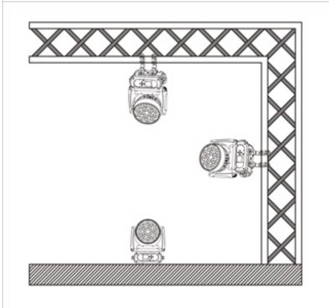
3.3 How to do mounting installation.
